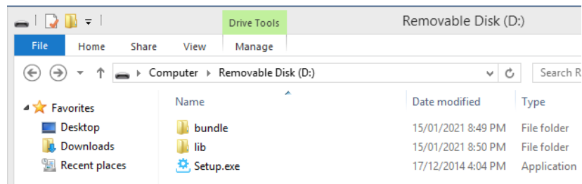
Figure 4 - Installation Files
