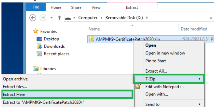
Figure 3 - Extract file
