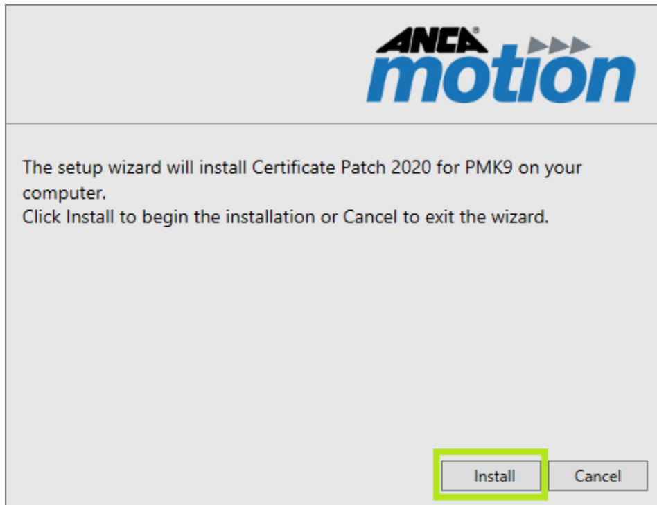
Figure 7 – Installation
