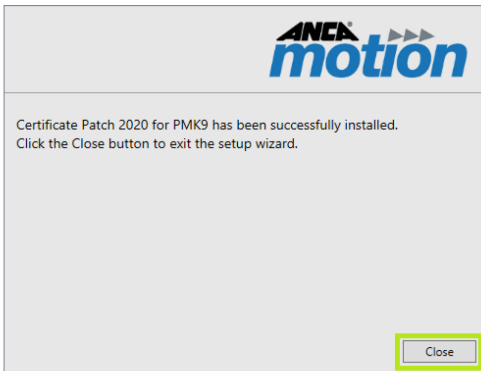
Figure 8 - Installation finish
