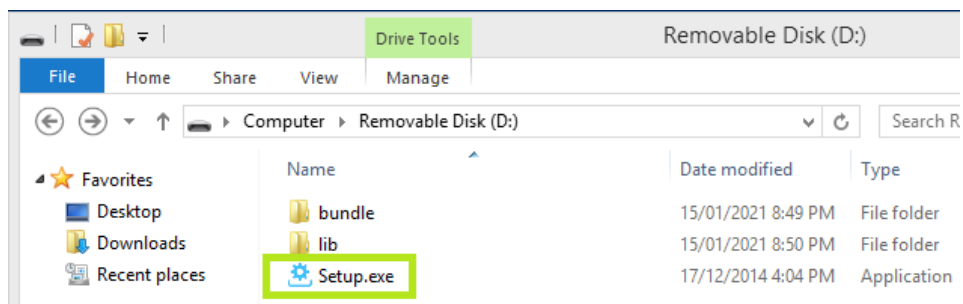
Figure 5 - Setup
