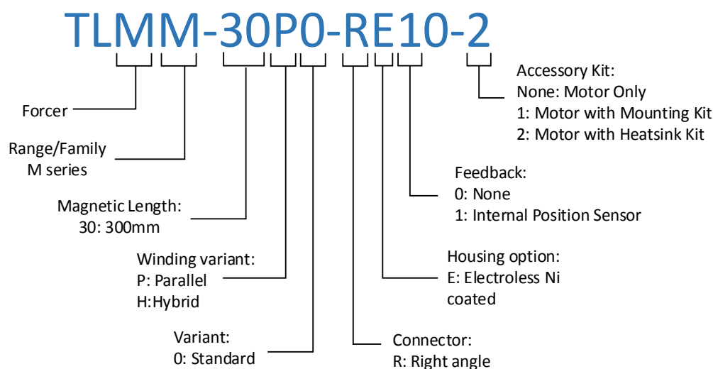
Figure 2-2 - Forcer catalogue number
