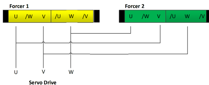
Figure 4-1 - Armature wiring diagram for parallel forcers
