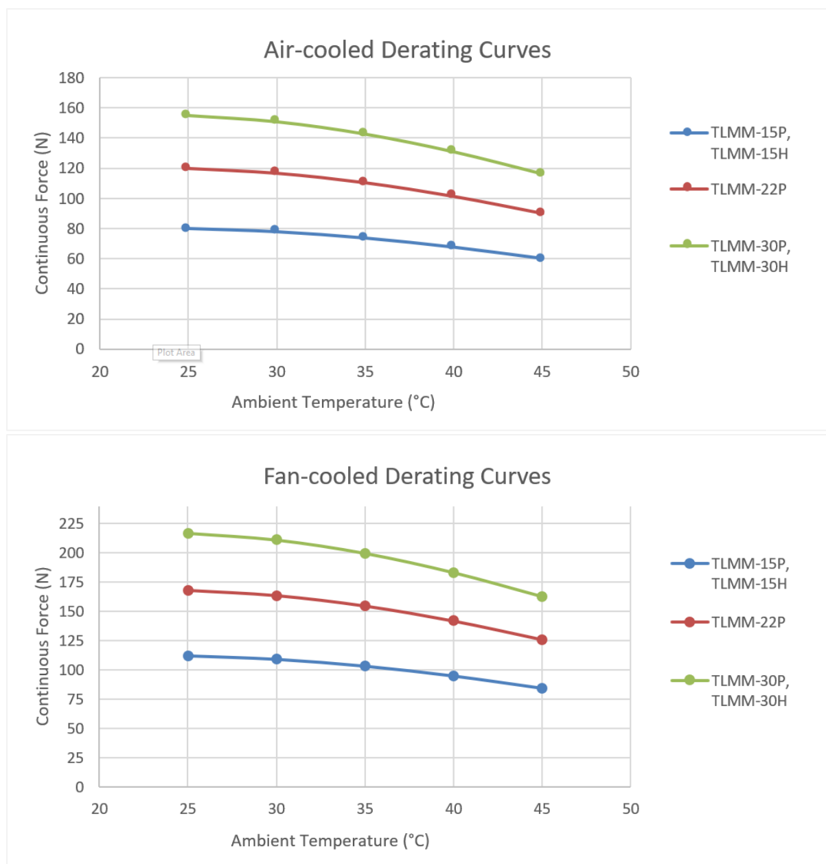
Figure 3-1 - Continuous Force derating with ambient temperature
