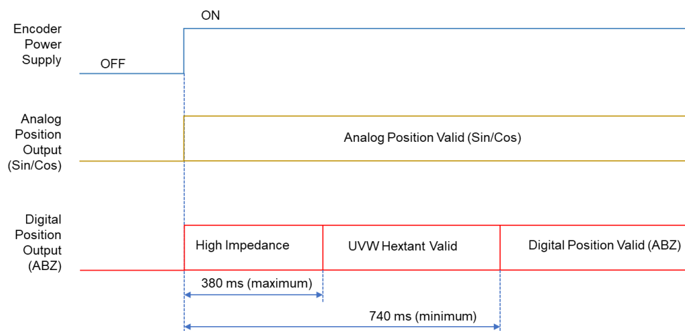
Figure 3-7 - ABZ channels start-up sequence timing diagram
