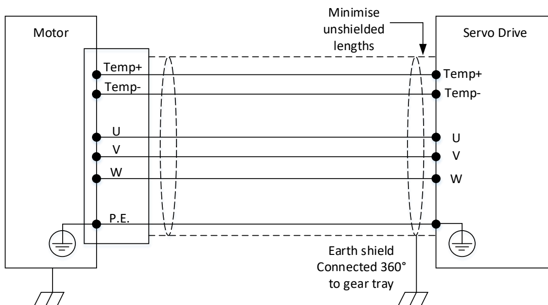
Figure 6-13 - Connection Between Motor and Servo Drive
