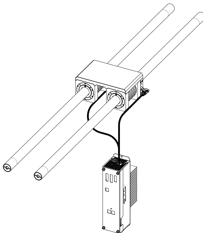
Figure 4-8 – Tandem Forcers
