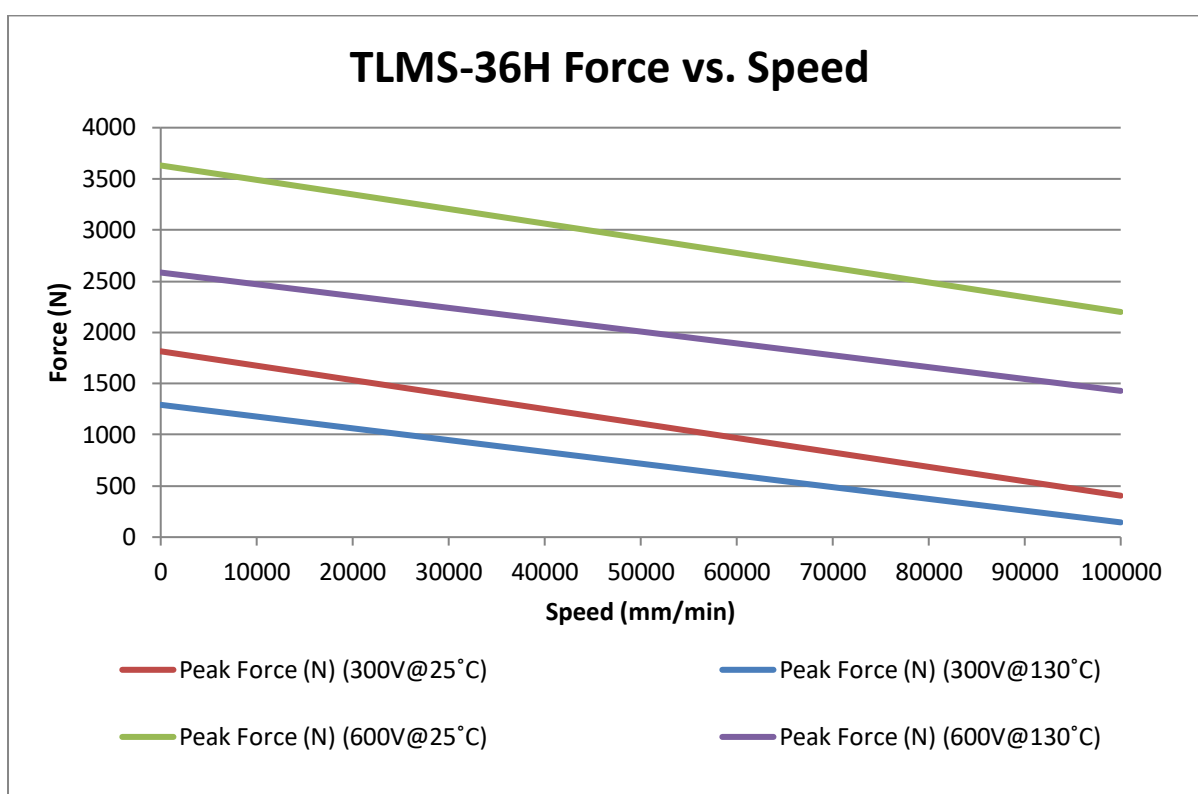
Figure 5-4 - TLMS-36H Peak Force vs. Speed
