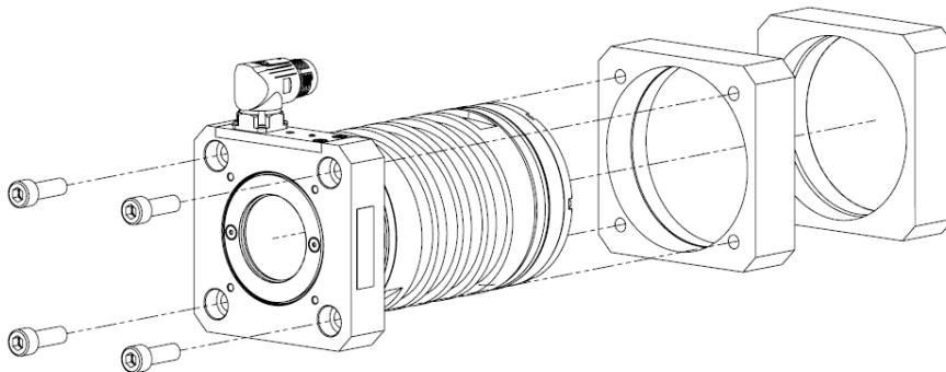
Figure 6-7 - Example of Air Cooled Forcer Mounting
