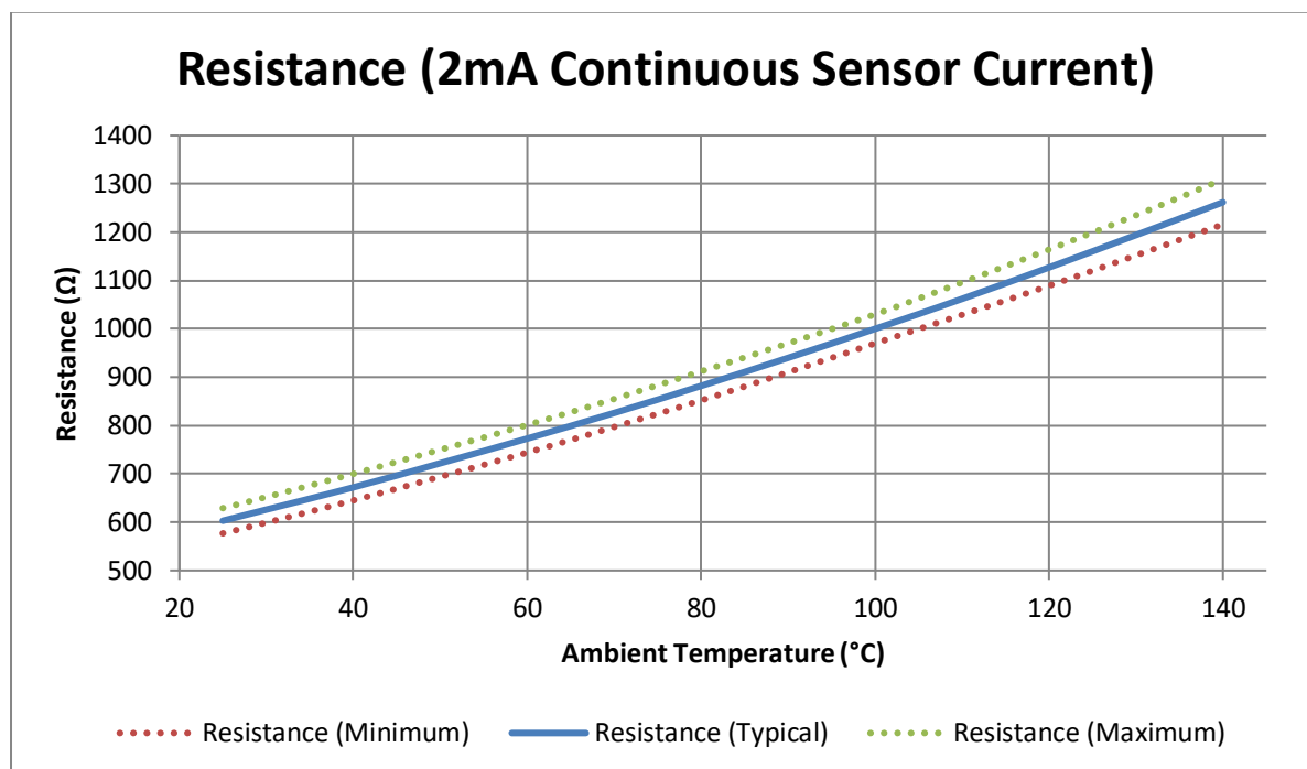
Figure 4-5 – KTY84/130 Temperature Sensor Characteristics
