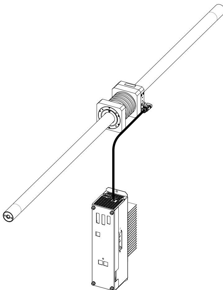
Figure 4-6 – Single Forcer
