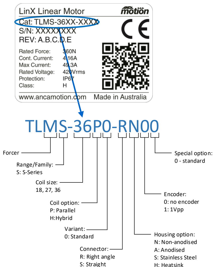
Figure 3-3 – Forcer Catalogue Number
