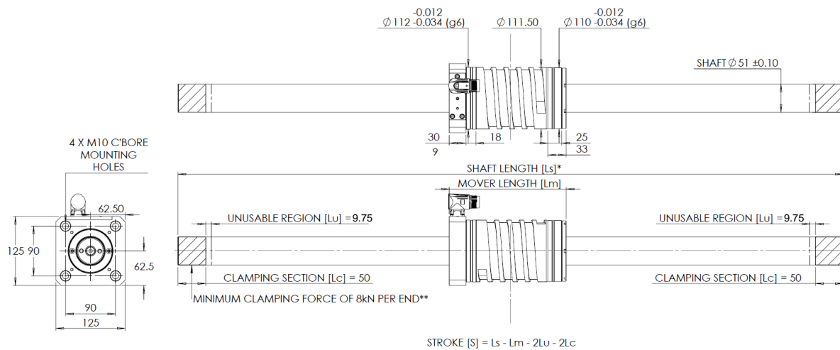
Figure 5-5 - Mechanical Dimensions
