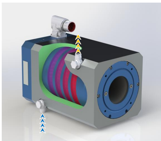
Figure 4-3 - Fluid cooled forcer mounting example
