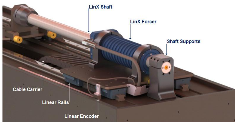
Figure 3-2 - The LinX System
