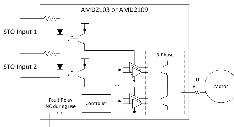
Figure 7-13 STO Implementation
