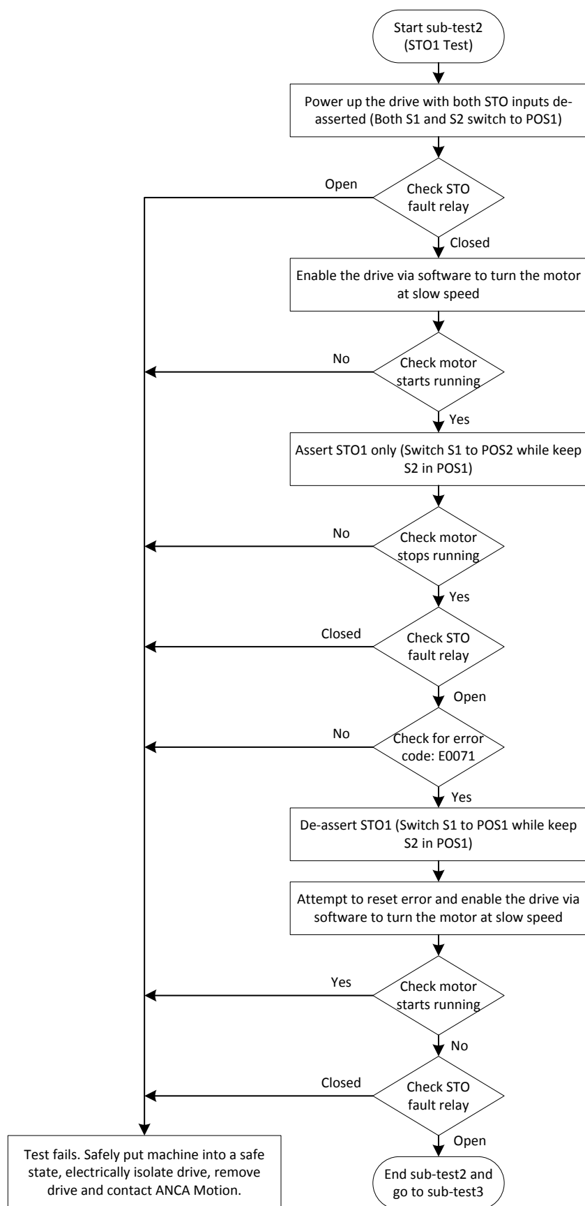
Figure 7-22 - STO Sub-Test 2
